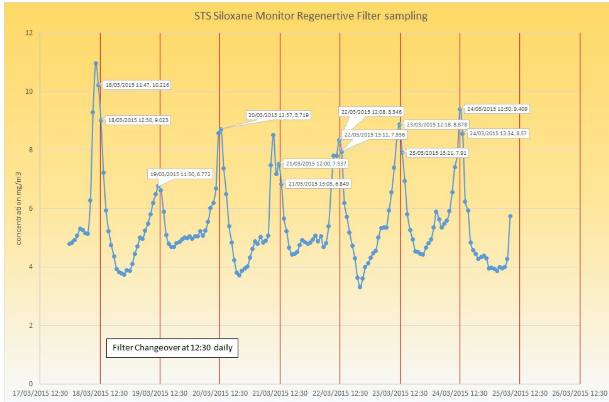
Daily Regenerative Filter results from AD Biogas Trial
